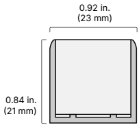
24V-3D-LIN-TW1840 in LINAIRE Flex 3D Bend Channel
