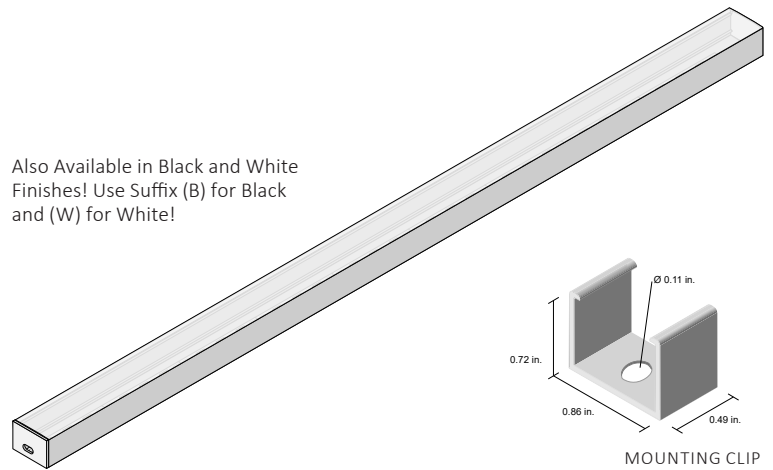
MOUNTING CLIP
